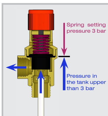
System pressure higher than the set pressure of the valve.
