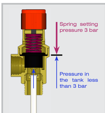
System pressure lower than the set pressure of the valve.
