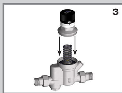
3- Re-assemble properly all components into reducer and screw again
