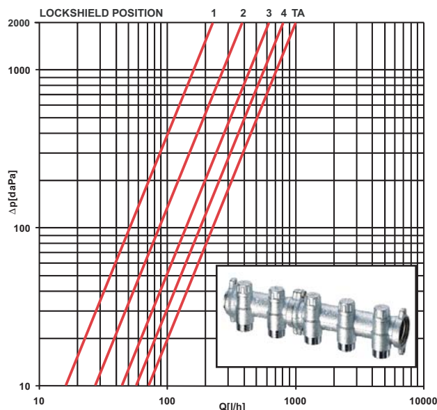
Art. 3915 1 thermoelectric flanged manifold with built-in lockshield valves
