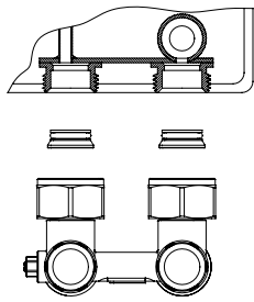
SECTIONED RADIATOR
