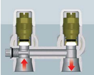
TOTALLY CLOSED BY-PASS: DOUBLE-PIPE VALVE
