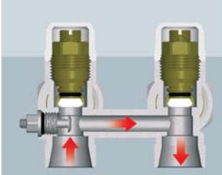
TOTALLY OPEN BY-PASS: SINGLE-PIPE VALVE
